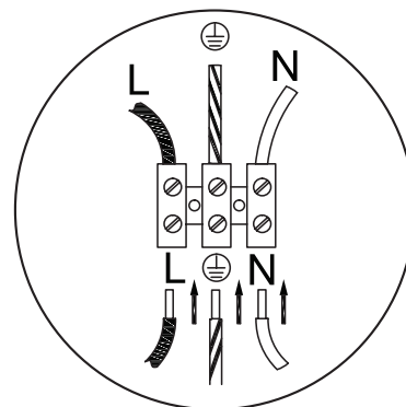
3. Details of terminal wiring.
