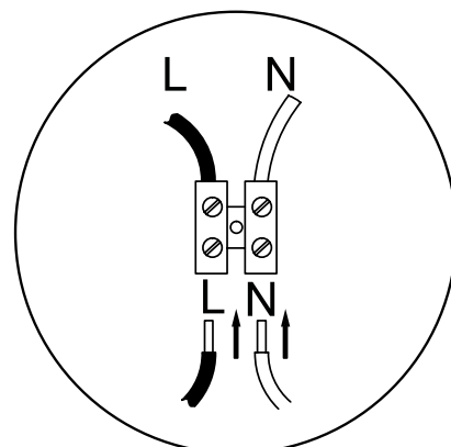
Class II - Double Insulated
