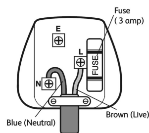
Plug wiring diagram
